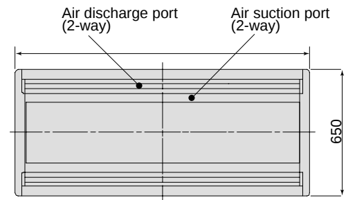
Z view
